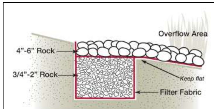
Figure 49: Rock Infiltration Set-up
